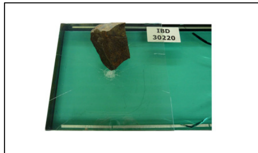
Protected Windshield after Stone-Chipping
