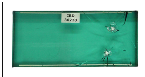
Windshield after Removal of Chipped DWP
